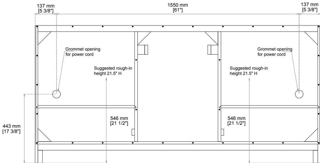
Back View
