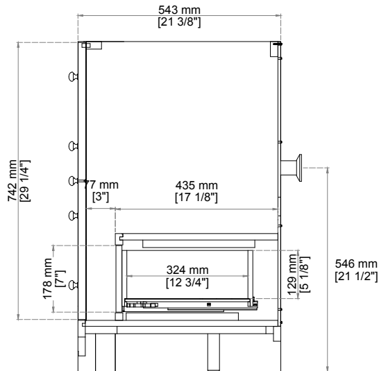
Side View 1
