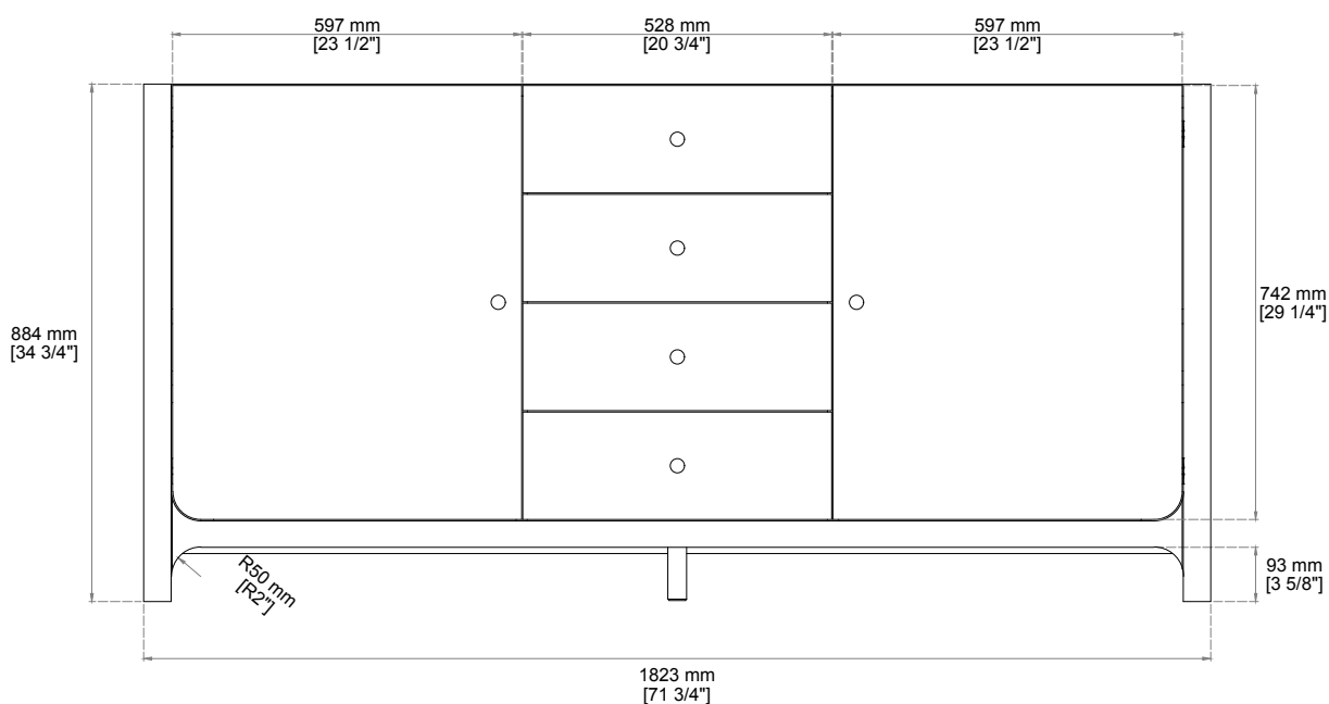
All dimensions are nominal Diagrams are of cabinet only. Optional Countertops and sinks are not shown.
