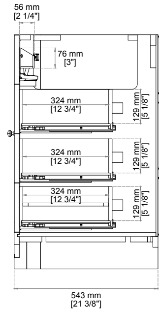
Side View 1
