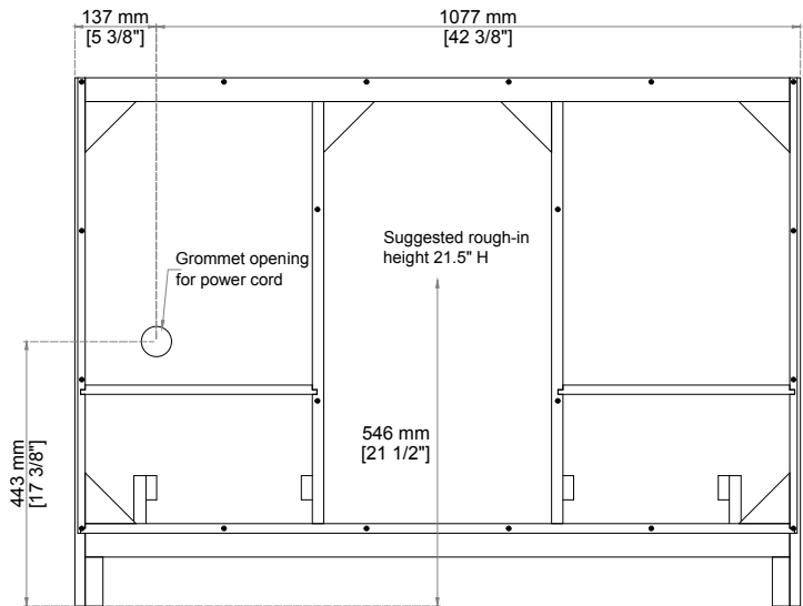
Back View
