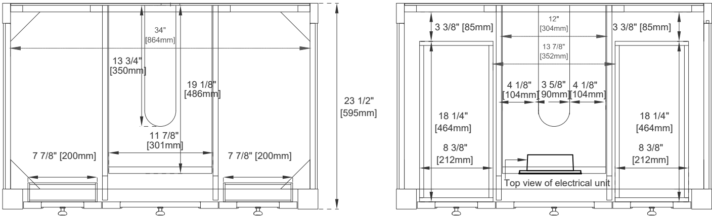
Top View
