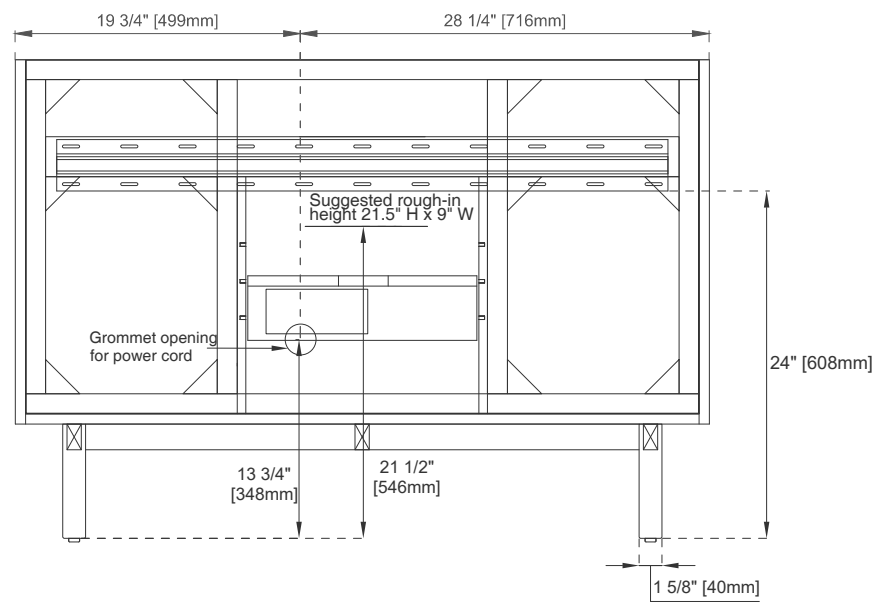
Back View
